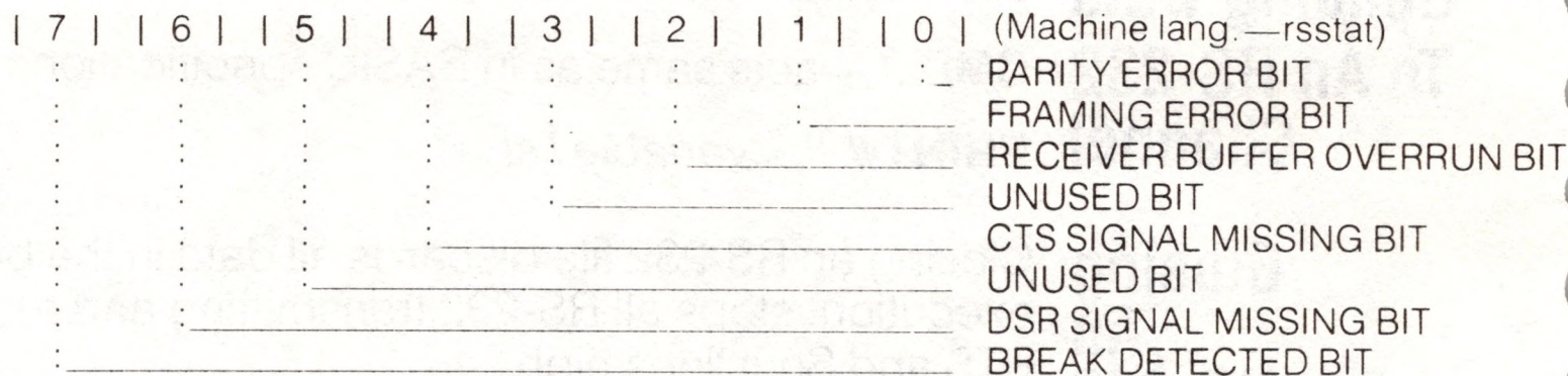
Figure A-3. RS-232 Status Register
